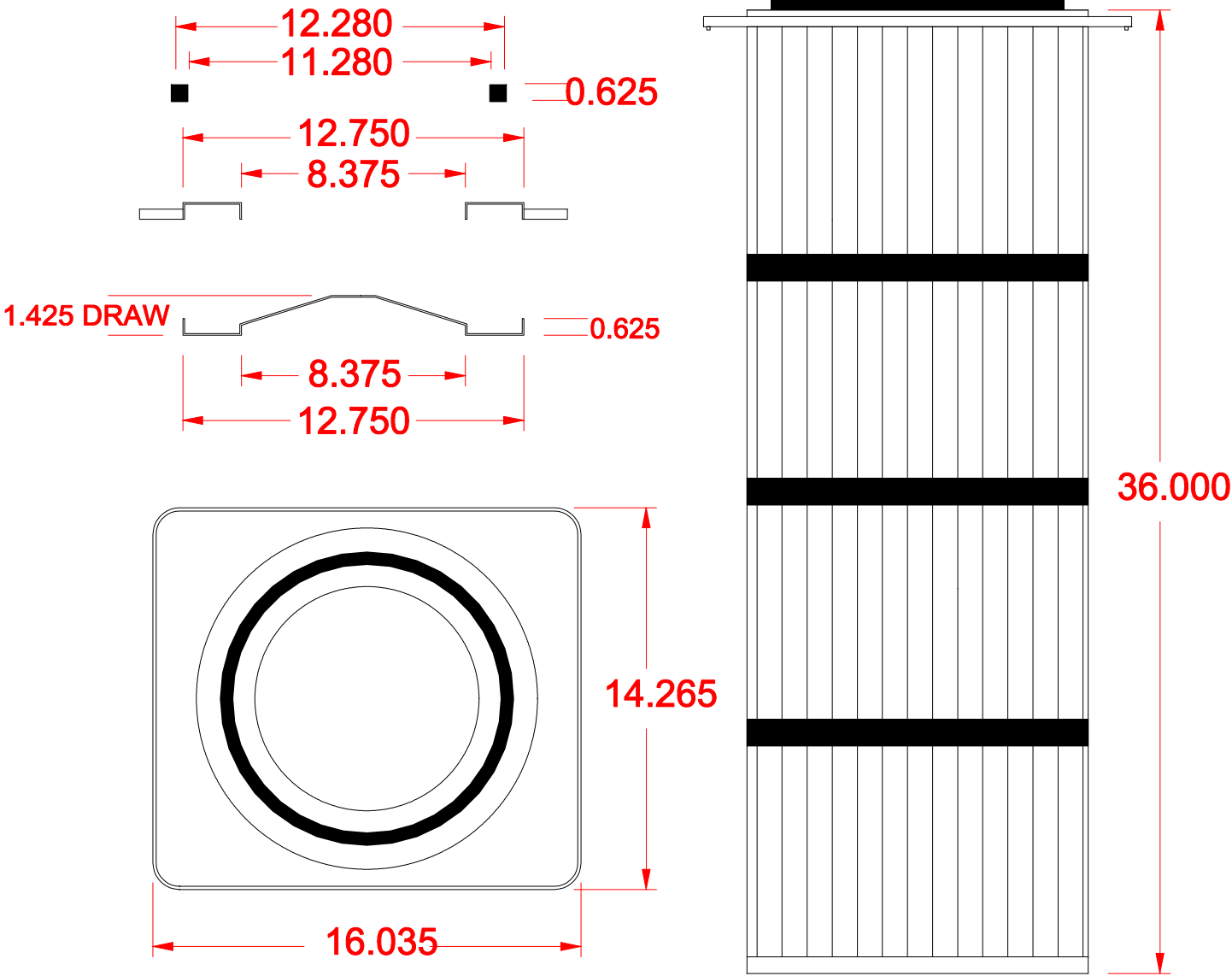
MERV 11 - 80/20 CELLULOSE / SYNTHETIC FIRE RETARDANT MEDIA
